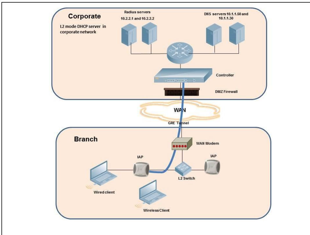
Figure 14 Scenario 4—GRE: Single Datacenter Deployment with No Redundancy
