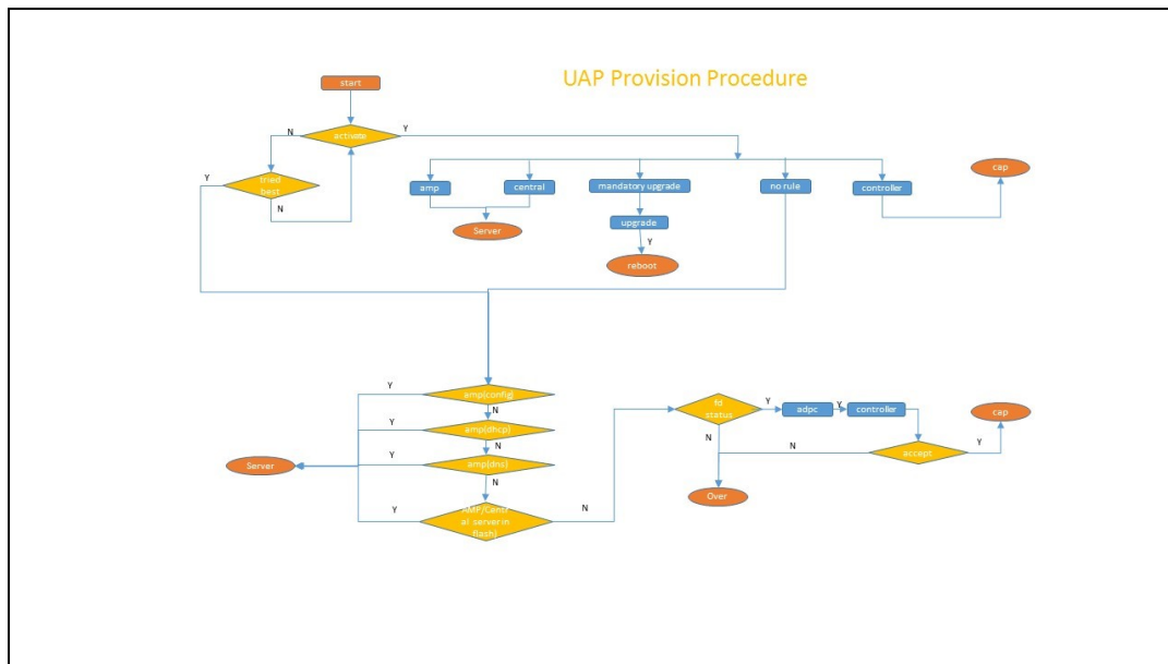
Figure 3 AP Discovery Logic
